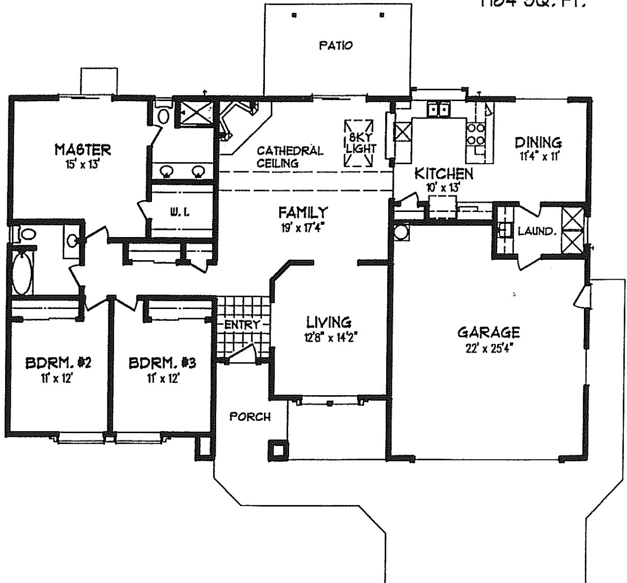
PLAN 424 1784 SQ. FT.
